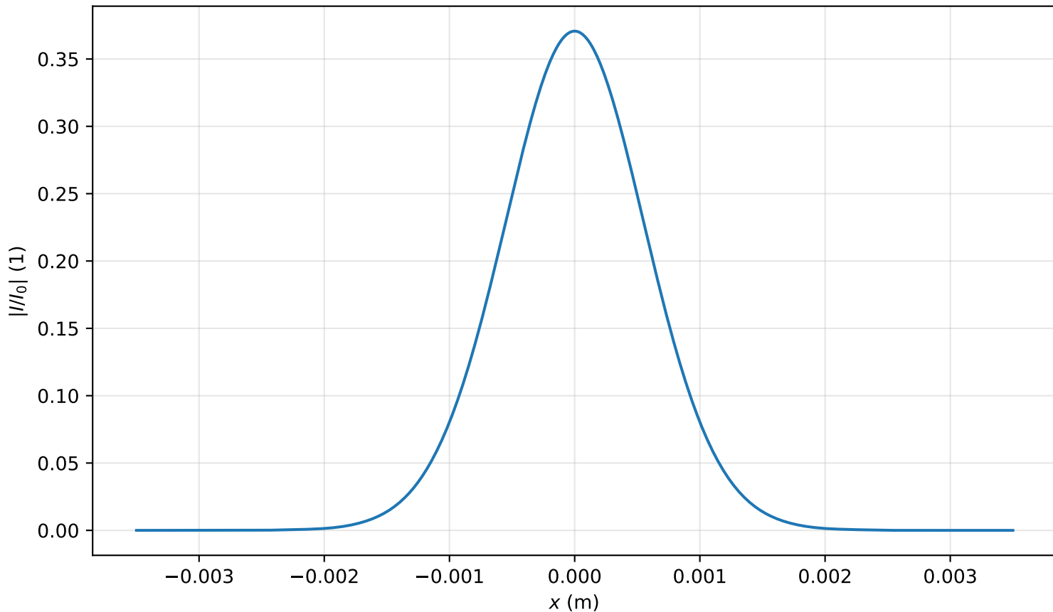
Intensity profile I(x, y = 0, z = 3.025m)/I_0 , P_{in}=0.2P_{cr} , artificial time
